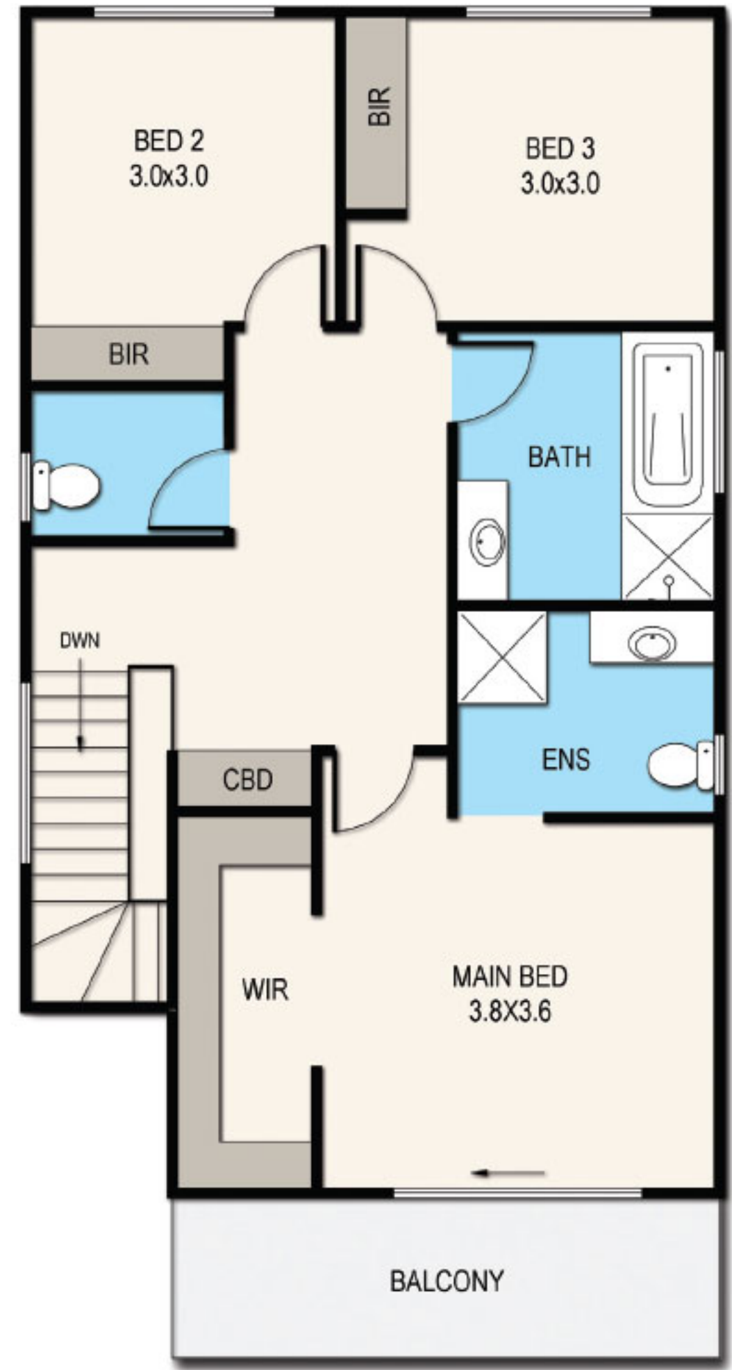
first floor
